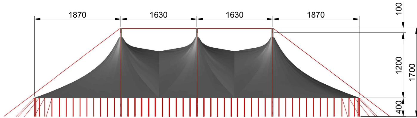
FRONT VIEW
